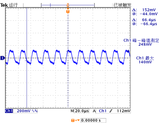
Figure 7, Output ripple & noise (Iout = 20A)
