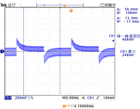
Figure 5, 50% - 75% load dynamic
