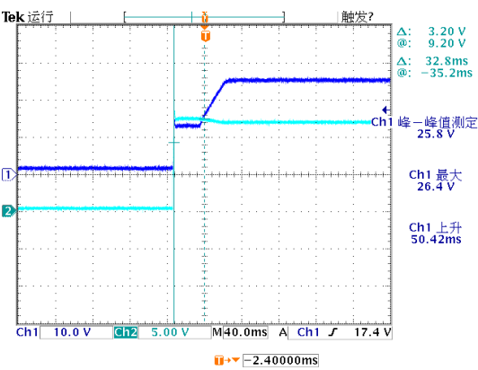
Figure 6, Output voltage established (Iout = 20A)
