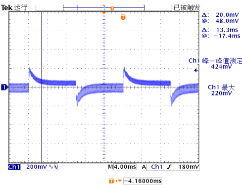
Figure 4, 25% - 50% load dynamic
